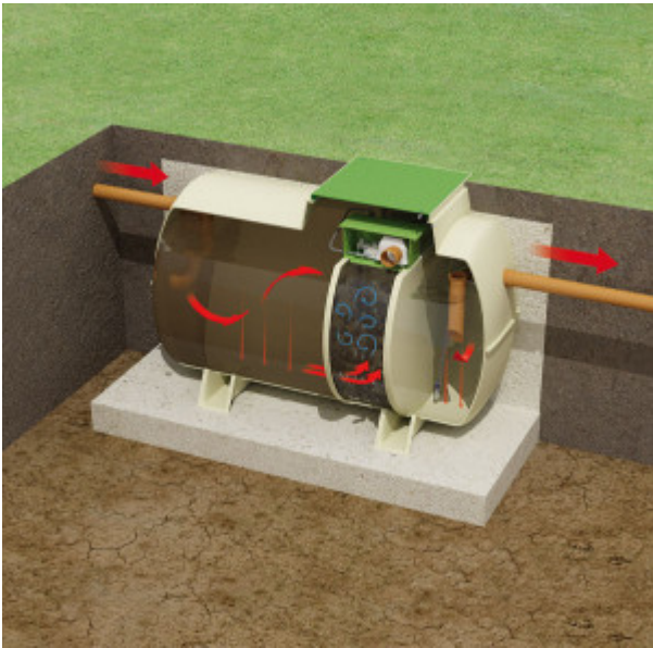
Septic Tanks and Sewage Treatment Plants
